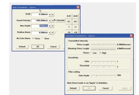
Basic and Customized Parameter Settings
