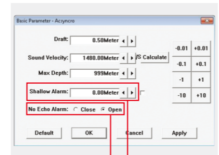
“No Echo” Alarm Shallow-water Alarm
